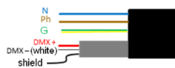
DMX cable
